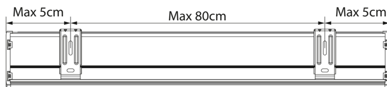
Inside mount
